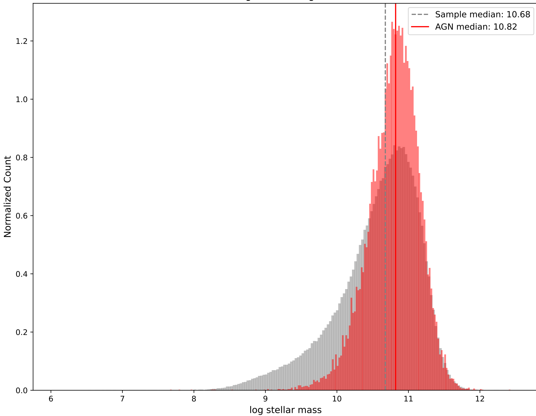
log Mass Histogram
