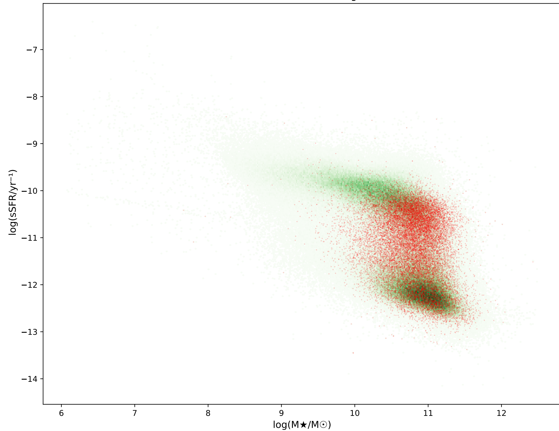
sSFR vs Stellar Mass diagram
