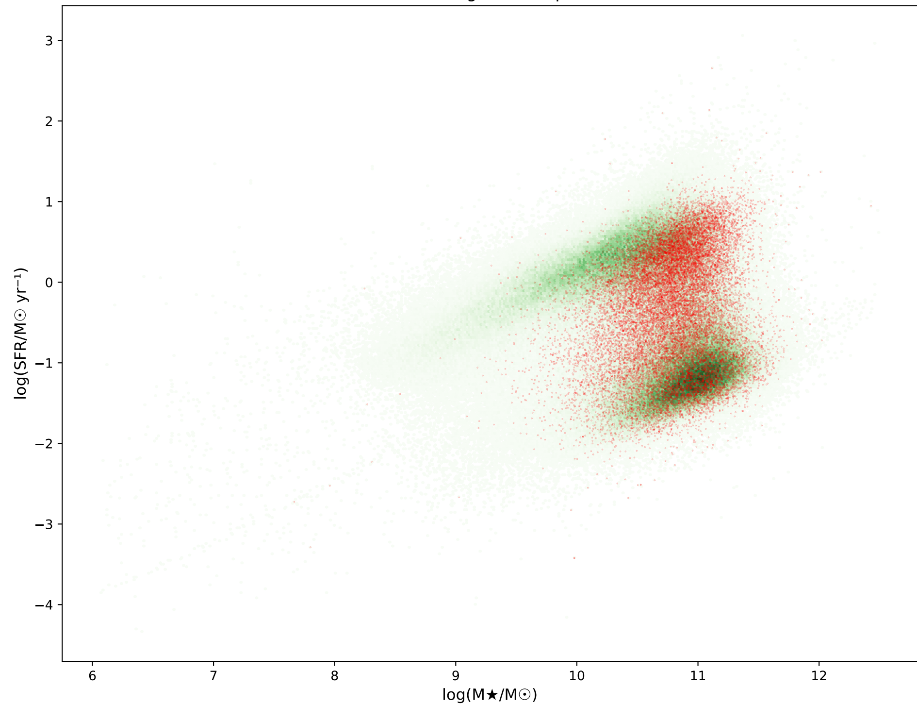
Star Forming Main Sequence
