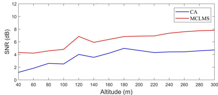
Figure 3.4: SNR after applying the CA and the MCLMS filter respectively
