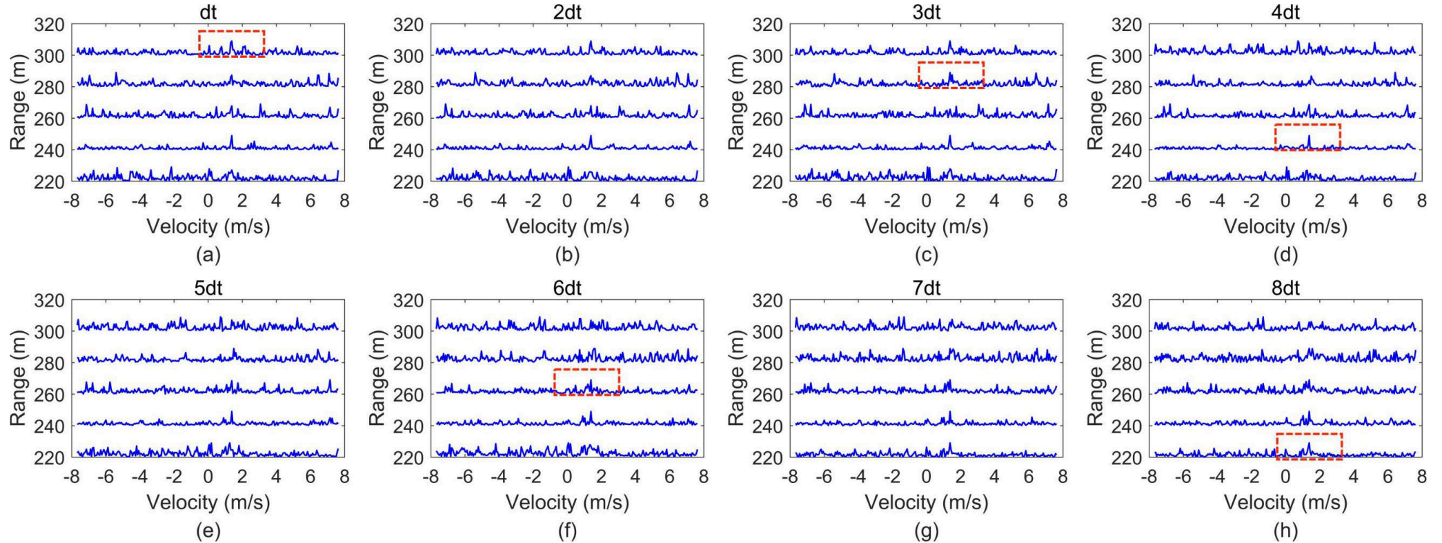
Fig: Optimal solutions are marked by red dotted box of different range bin after mutual convolution (a)–(h) Represent the filtering effect of dt – 8dt delay time respectively.
