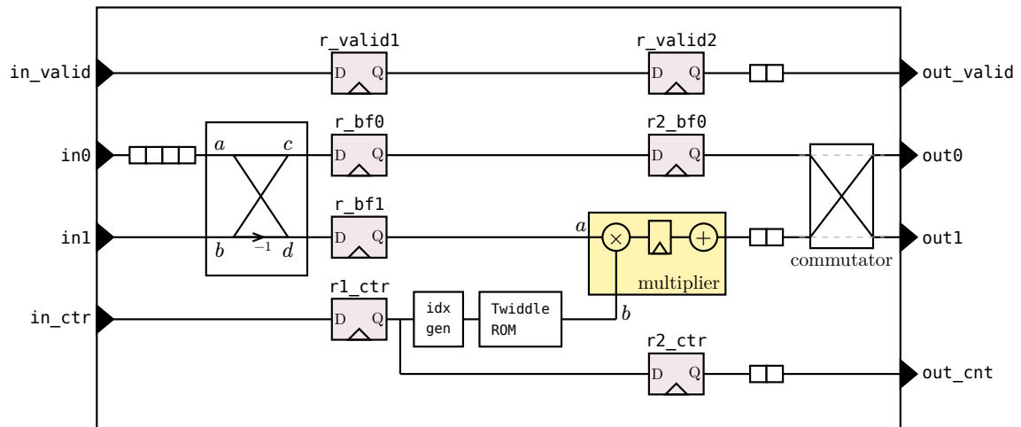
Figure 1.9: Inside a single R2MDC Stage. All modules with wedge is clocked
