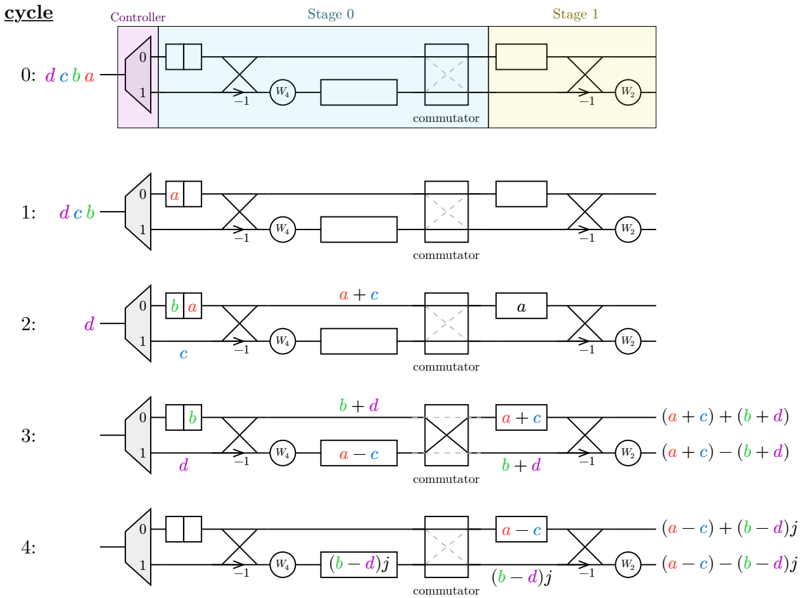
Figure 1.7: Steps in R2MDC algorithm with N = 4 case
