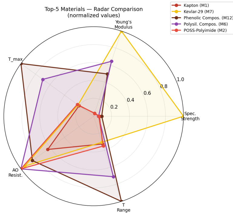
Figure 7. Multi-criteria radar comparison of the Top-5 candidate materials (normalised values, max = 1.0).
