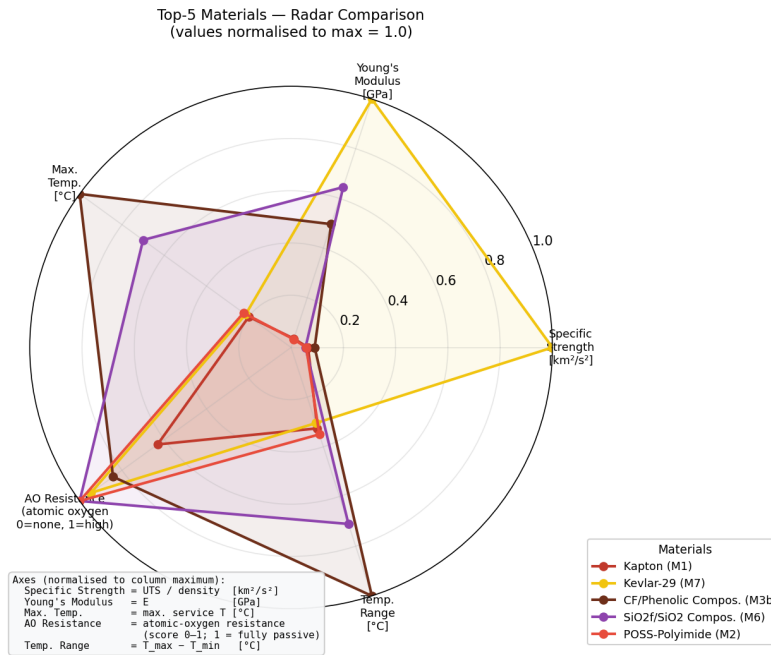
Figure 7. Multi-criteria radar comparison of the Top-5 candidate materials (normalised values, max = 1.0).
