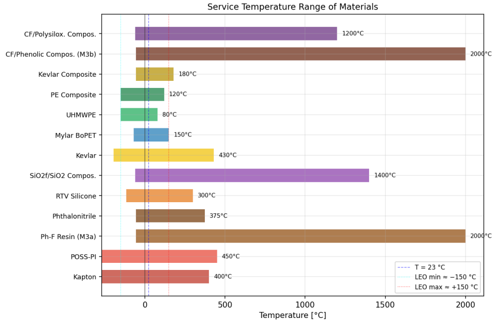
Figure 6. Service temperature range of M1–M13. Dotted lines mark the LEO thermal envelope (–150 to +150 °C).
