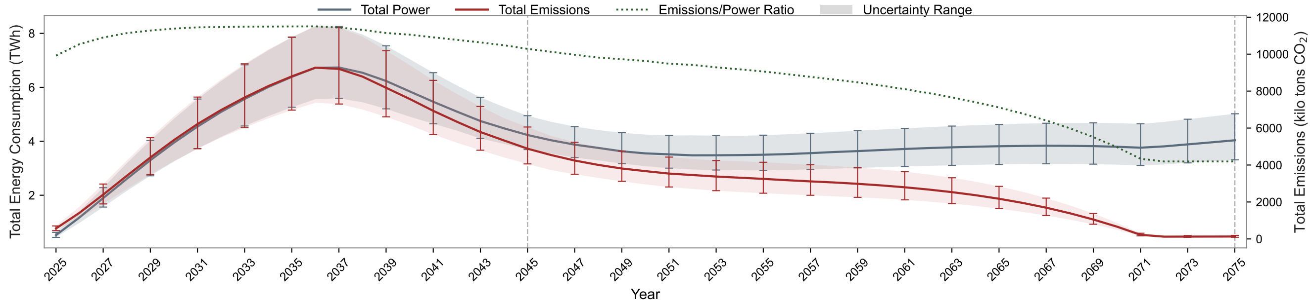
Annual ATS Energy Consumption and Emissions Prediction for California (2025–2075)
