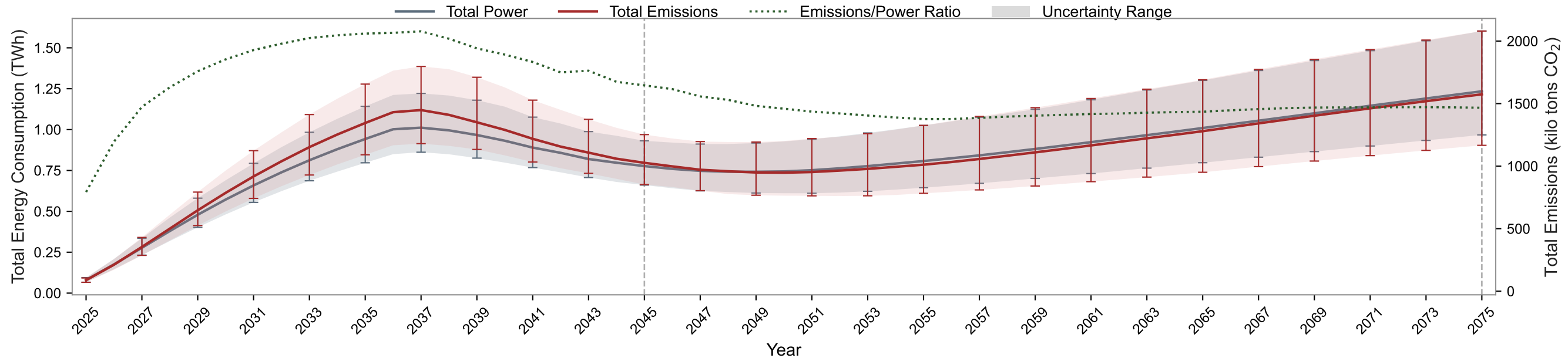
Annual ATS Energy Consumption and Emissions Prediction for Ohio (2025–2075)
