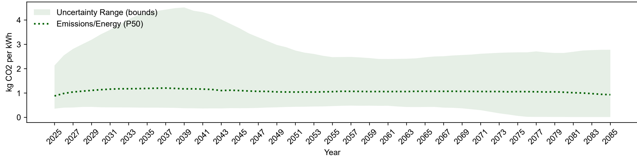
Emissions/Energy Ratio for California (2025-2085)
