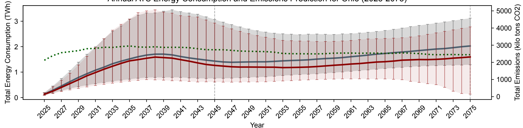
Annual ATS Energy Consumption and Emissions Prediction for Ohio (2025-2075)
