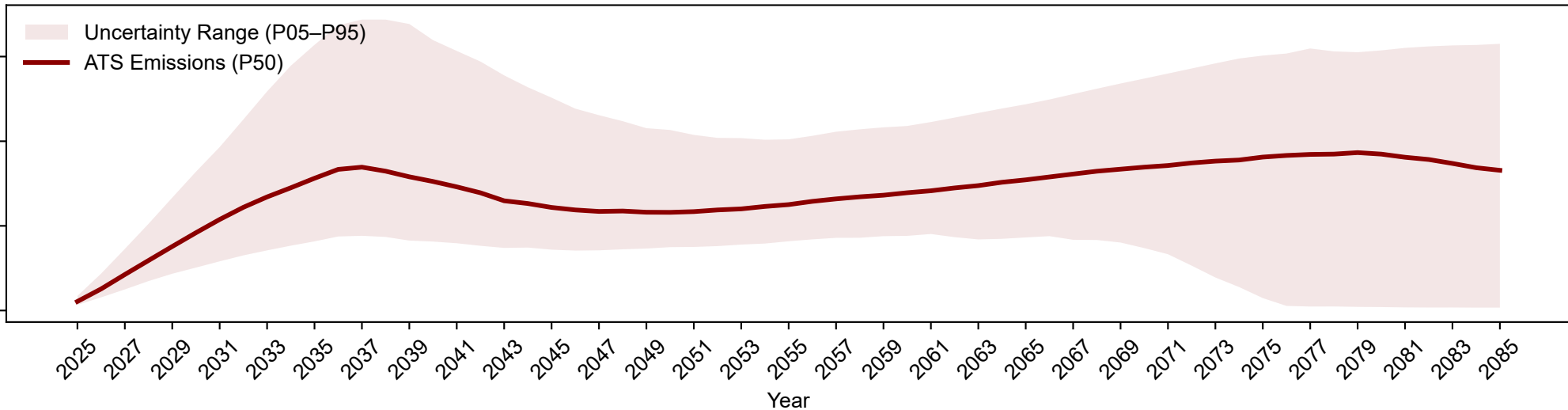
ATS Emissions Prediction for California (2025-2085)
