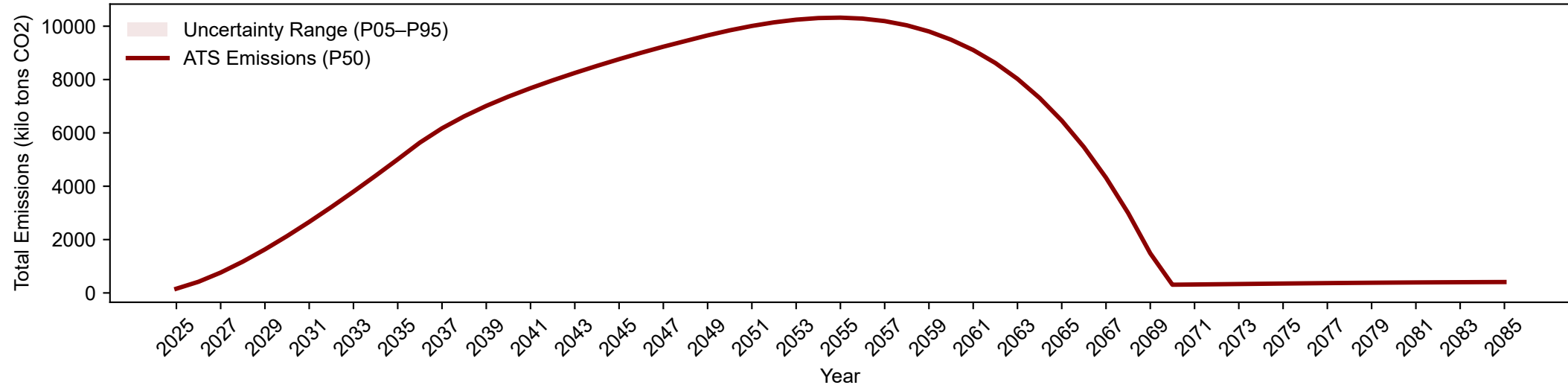
ATS Emissions Prediction for US average (2025-2085)
