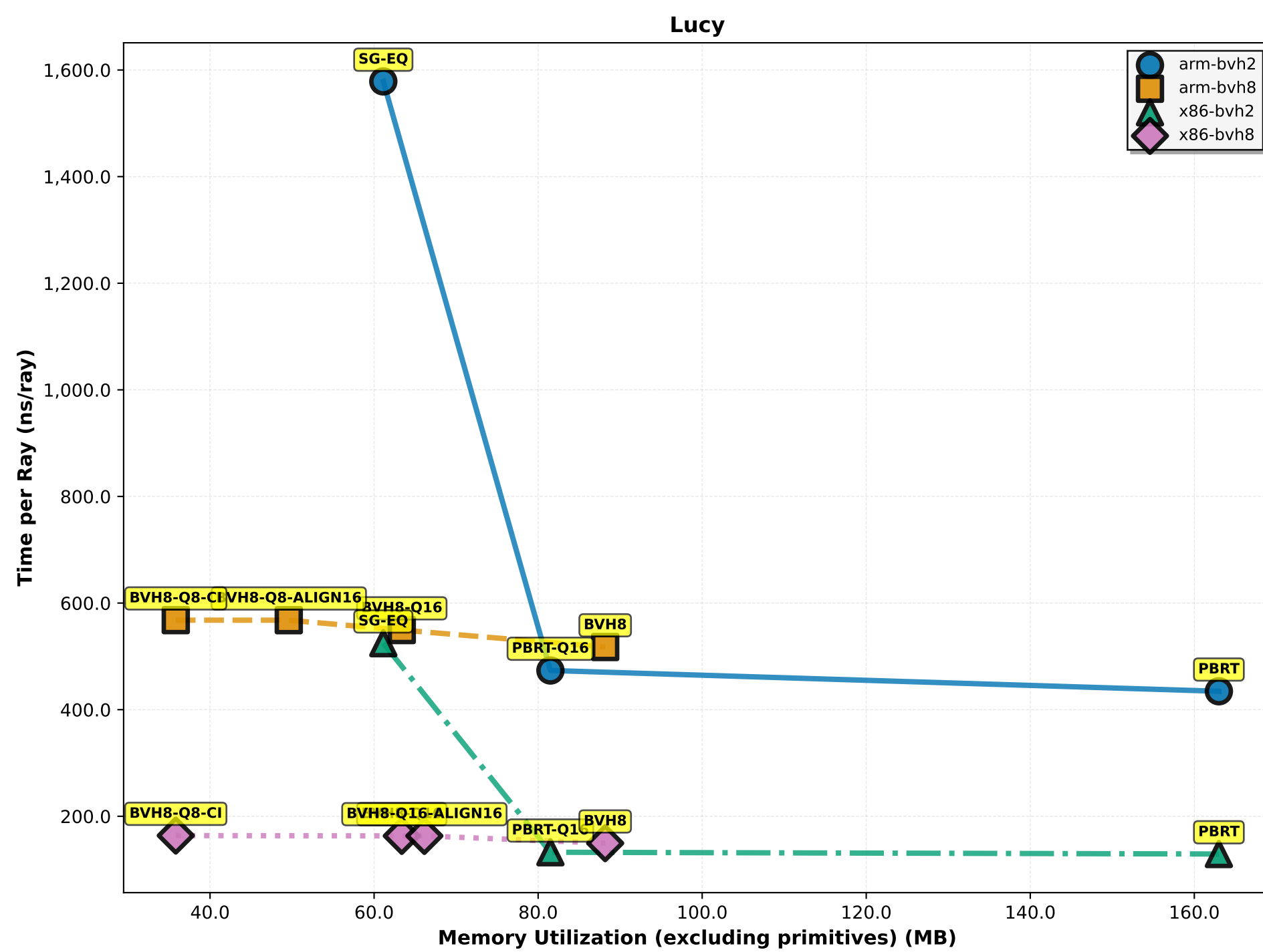
Time per Ray vs Memory Utilization wavg (all) - x86,arm - secondary
