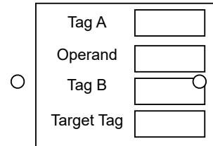
Compute
