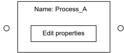
Process
