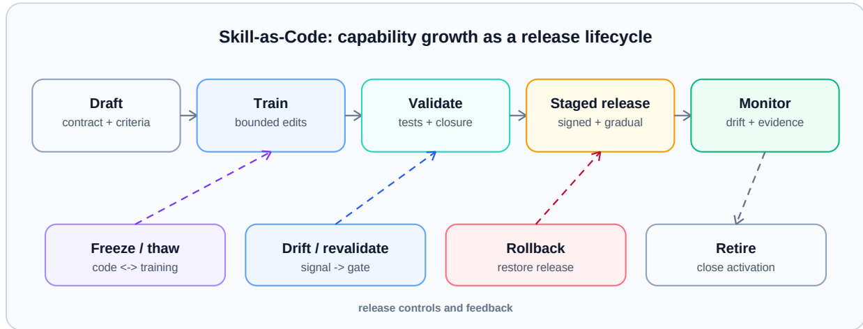
Figure 7. Skill-as-Code lifecycle. A candidate moves through draft, training, validation, staged release, and monitoring. Drift triggers revalidation; operators may freeze or thaw a Skill, roll back a staged or active release, and retire an identity while retaining lifecycle continuity and audit evidence.
