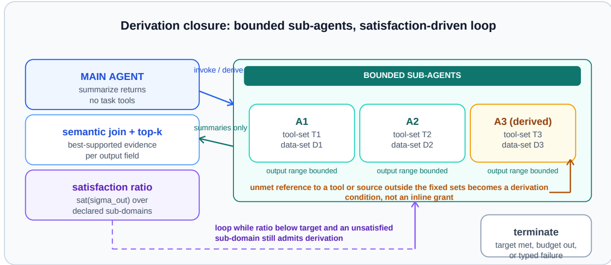
Figure 4. Derivation-closure orchestration. Each sub-agent holds an admitted tool-set and data-set; references outside those sets become conditions for deriving a new sub-agent rather than being granted inline. The main agent summarizes returns, performs a semantic join with top-k selection, and reports a satisfaction ratio computed by version-bound per-domain verifiers. Only deterministic or calibrated, version-pinned verifier results may participate directly in termination; other scores remain estimates requiring an independent gate.
