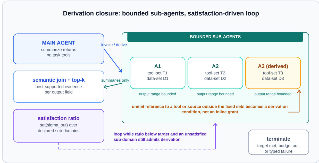
Figure 4. Derivation-closure orchestration. Each sub-agent holds a fixed tool-set and data-set, which bounds its output range; references to tools or sources outside that set become admission conditions for deriving a new sub-agent rather than being granted inline. The main agent summarizes returns, performs a semantic join with top-k selection, and measures the satisfaction ratio over the declared output sub-domains, iterating until the target is met or no derivation candidate remains. Capability discovery within a request thus proceeds by bounded derivation under the same deterministic gates as any other contract compilation.
