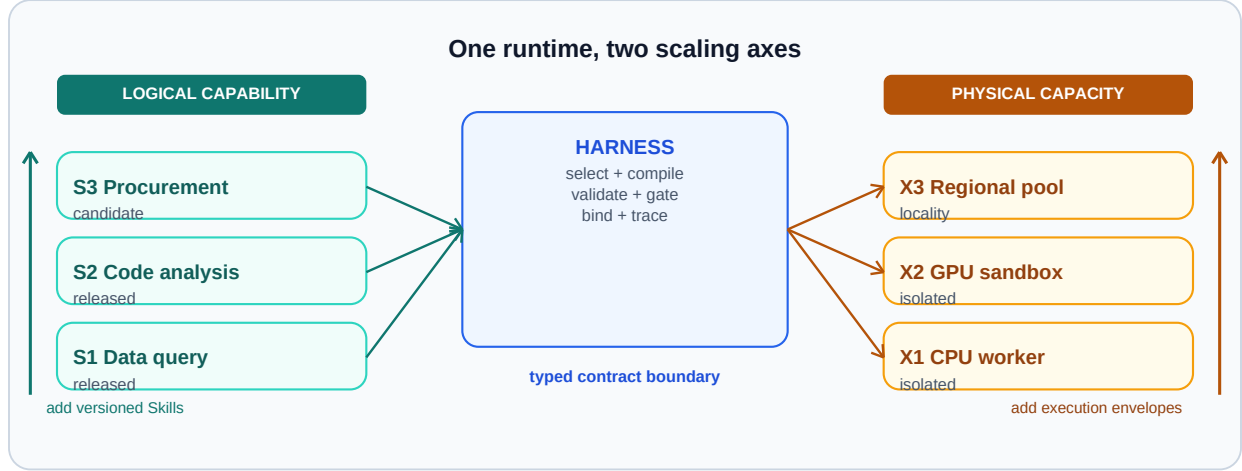
Figure 1. Dual scaling model. Logical extension adds or revises Skills through the Harness contract; physical extension adds Scaffold capacity through the same binding boundary. The architecture makes capability growth and capacity growth distinct interventions whose separability can be tested inside a declared operating region.
