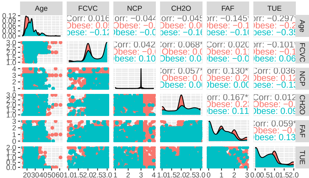
Pairwise Scatterplots of Continuous Variables by Obesity Class
