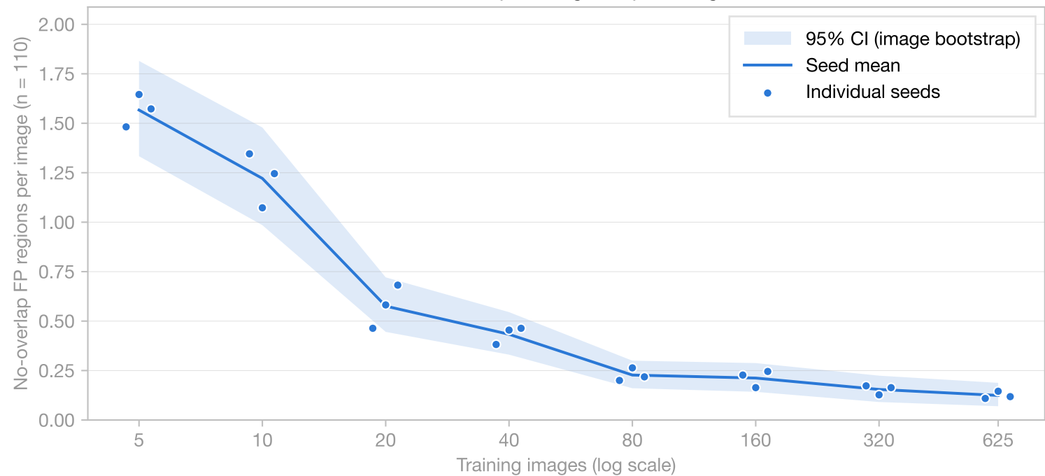
No-overlap FP regions per image
