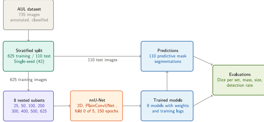
Figure 2: Study pipeline. The AUL dataset is split into fixed test and training sets, with nested subsets drawn from the training set. Each subset trains an independent nnU-Net model evaluated against the same test set.
