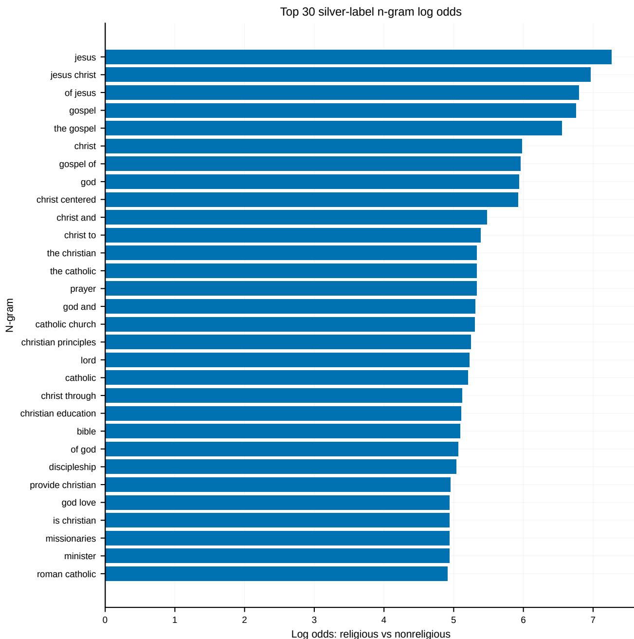
Figure B11 — ngram_log_odds. Top-30 naive signed n-gram log-odds (a simple aggregate precursor to the prior-shrunk weighted version in Figures B15–B17). Descending: jesus (~7.3), jesus christ , of jesus , gospel , the gospel , christ , god , christ centered , then catholic , prayer , bible , discipleship , missionaries . Conclusion: the classifier keys on intuitive, face-valid Christian/Catholic vocabulary; the weighted diagnostics that follow confirm the same ordering with a rigorous statistical prior.
