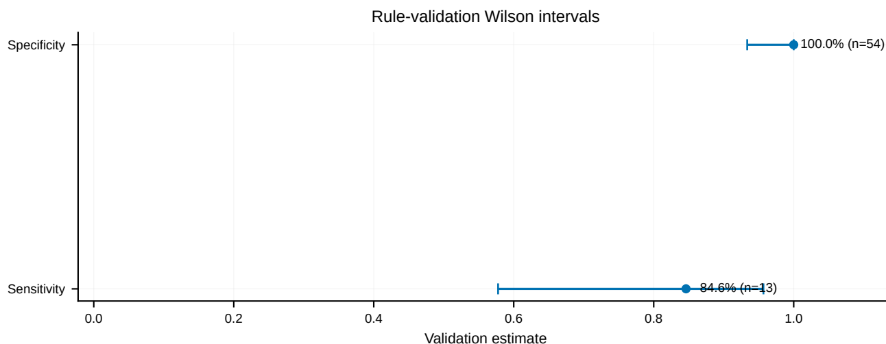
Figure B8 — rule_validation_intervals. Dot-and-whisker Wilson intervals for the LOW-tier rule. Specificity 1.00 (n=54, lower bound ~0.93); sensitivity 0.846 (n=13, CI ~0.58–0.97). Conclusion: the rule is highly specific but its recall is uncertain on a tiny positive sample — the driver of the wide LOW-tier band.
