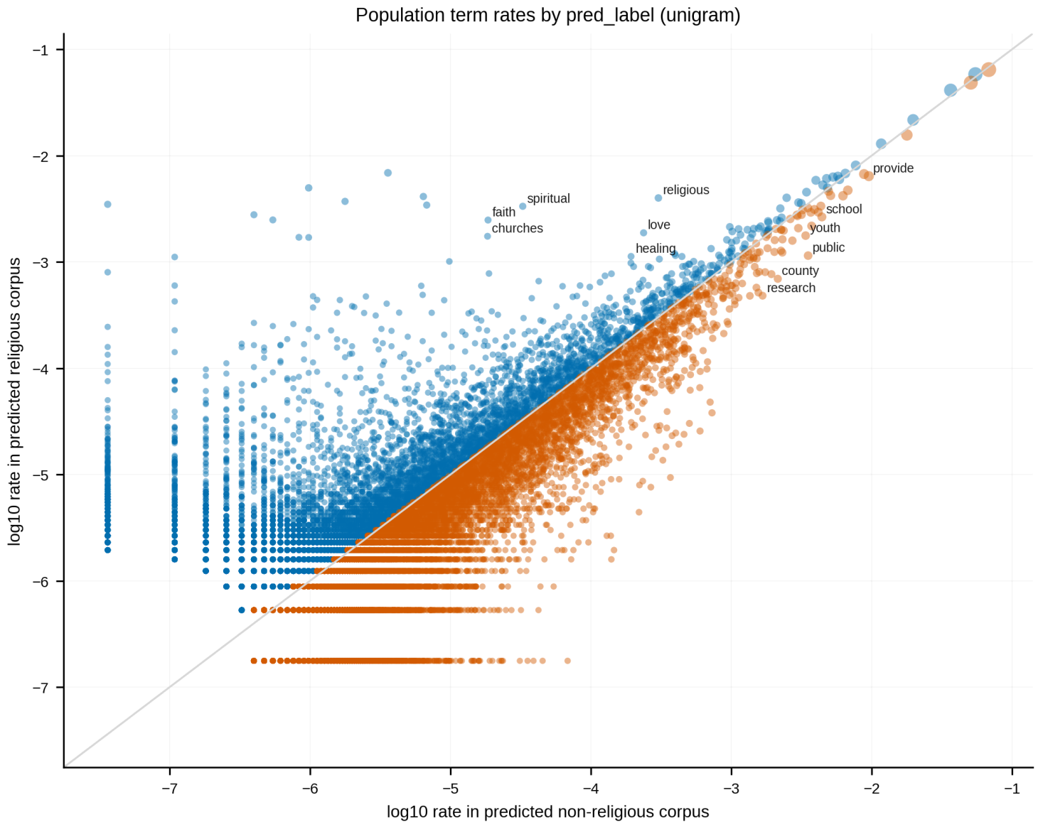
Figure B23 — population_term_scatter_{pred_label,pred_label_maxf1,pred_label_baserate}_unigram , population_term_scatter_pred_label_bigram . Four diagnostic panels (no trigram and no probability-weighted variant). Each plots a term's \log_{10} rate in the predicted-non-religious corpus against its \log_{10} rate in the predicted-religious corpus, with a grey identity diagonal, so that a term's perpendicular distance from the diagonal is its log rate ratio and the labelled outliers are the same ones the volcano labels — religious, spiritual, faith, churches, love, healing above the line, public, provide, county, research, school, youth below it. It surfaces no term the volcano does not, it is noisy at roughly 30,000 plotted unigrams, and the discretization floor of the low-count terms shows as horizontal and vertical striping in the lower left. Conclusion: retained for completeness as a direct view of the two class rates, but Figure B20 is the panel to read. A practical note: the SVG renderings of this family are very
