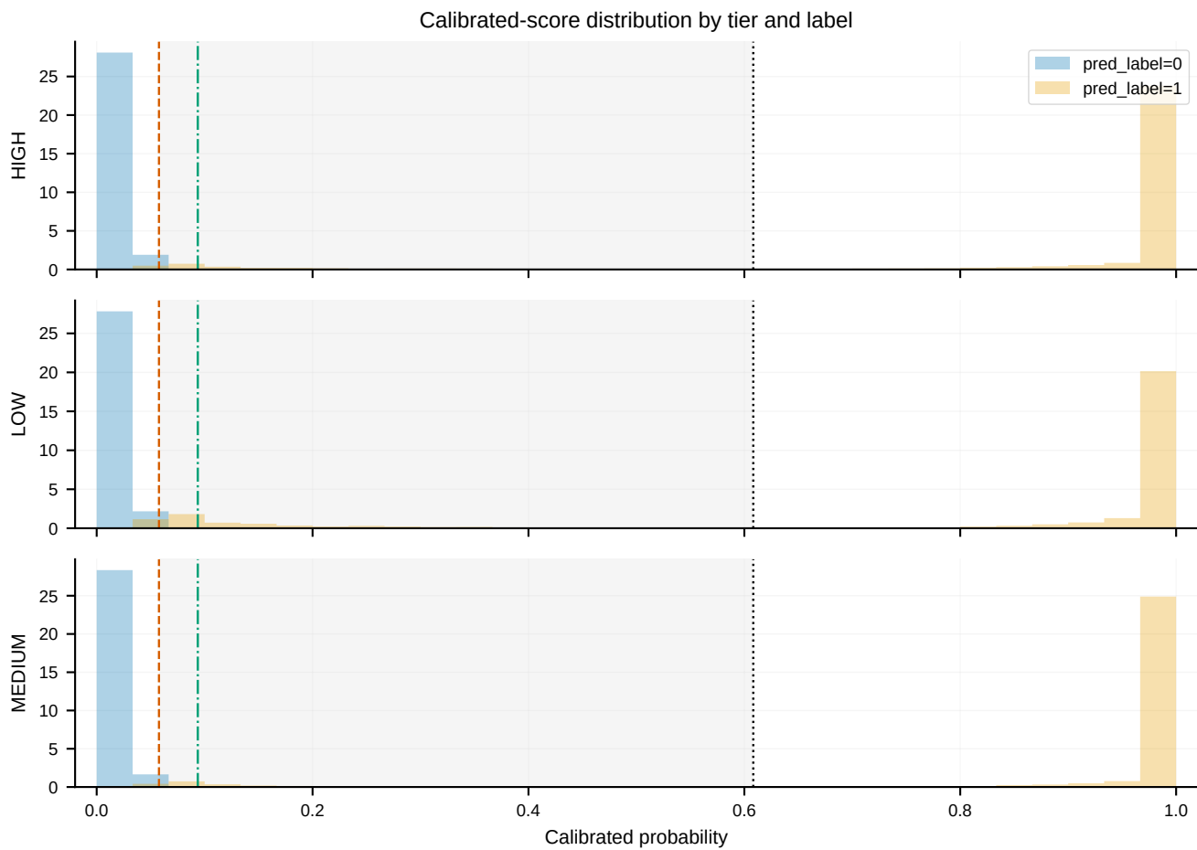
Figure B4 — score_distribution_by_tier_label. Stacked histograms of calibrated probability by tier (HIGH/MEDIUM/LOW), colored by predicted label, with the three thresholds and the inter-threshold band marked. Sharply bimodal in every tier (spikes near 0 and near 1). Conclusion: classification is insensitive to exact threshold placement within the wide gap; LOW shows marginally more mid-range mass.
