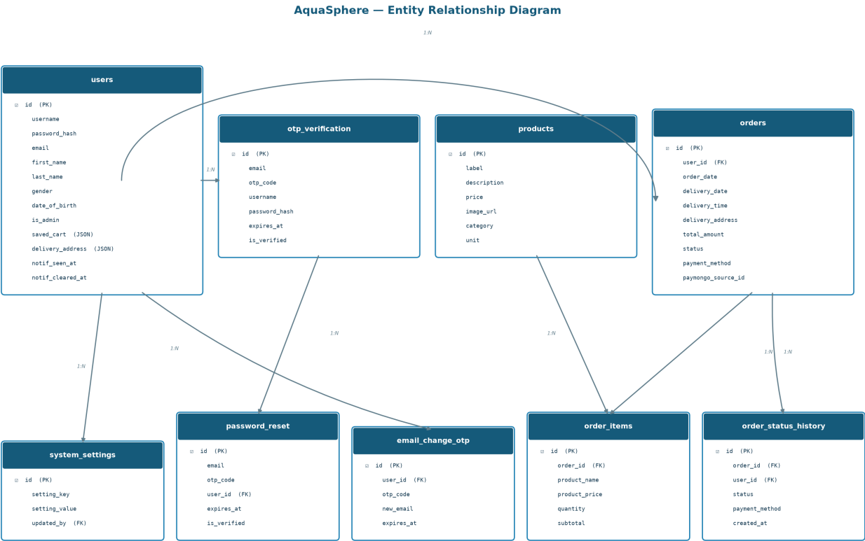
Figure 1. Entity Relationship Diagram showing core tables and their relationships.
