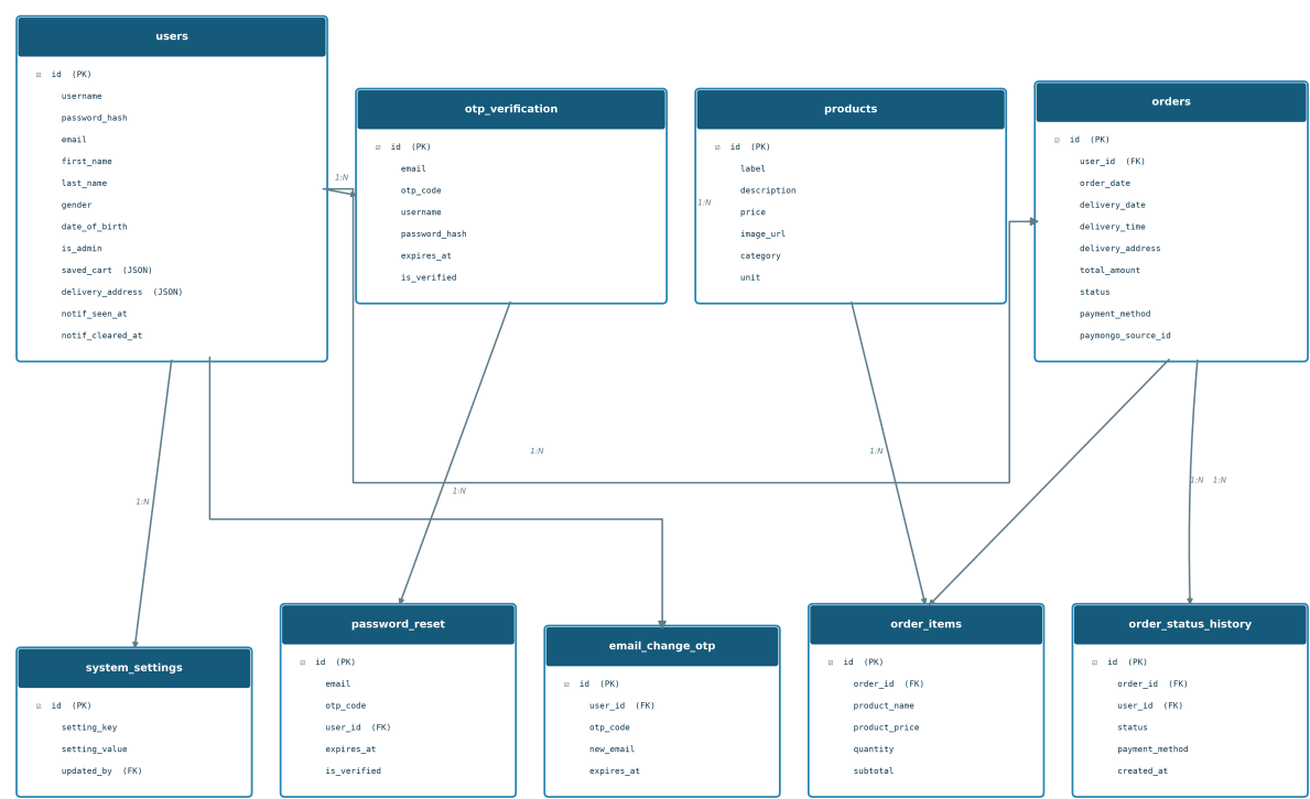
Figure 1. Entity Relationship Diagram showing core tables and their relationships.
