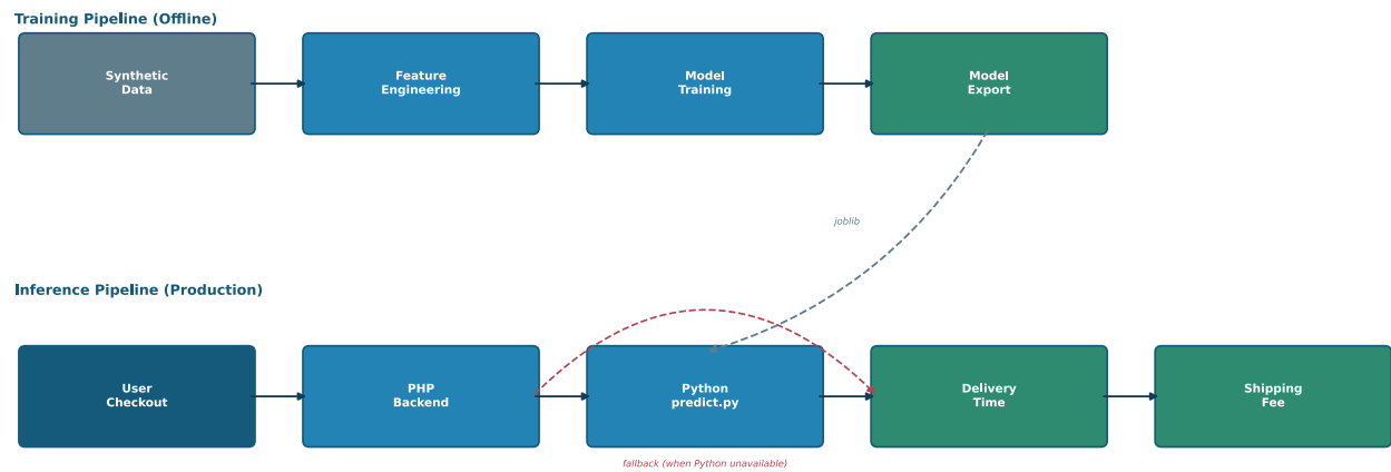
Figure 2. ML training and inference pipeline.
