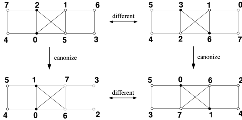
Figure 3.3: Example of GI with canonical labelling from [43]
