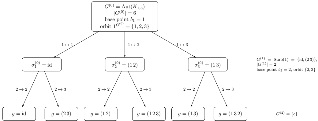
Figure 4.3: Tree associated with the BSGS of \text{Aut}(K_{1,3}) with base (b_1 = 1, b_2 = 2) .
