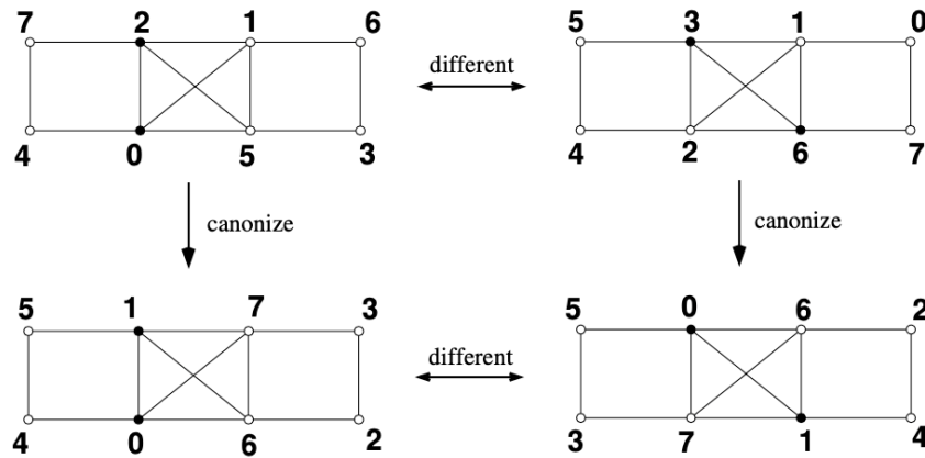
Figure 3.2: Example of GI with canonical labelling from [47]
