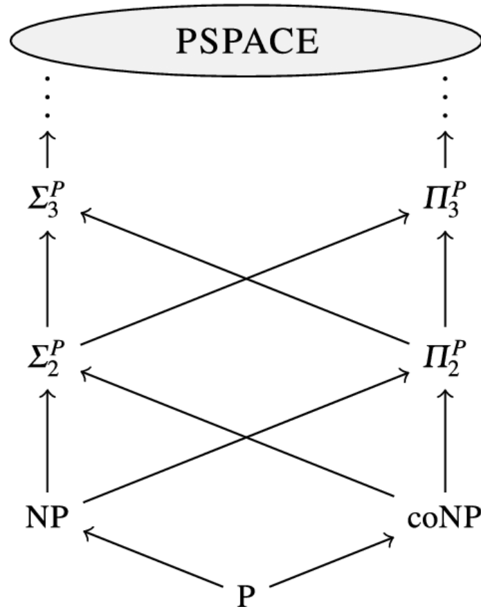
Figure 2.2: Polynomial Time Hierarchy where the arrows denote the inclusion: image from [7]
