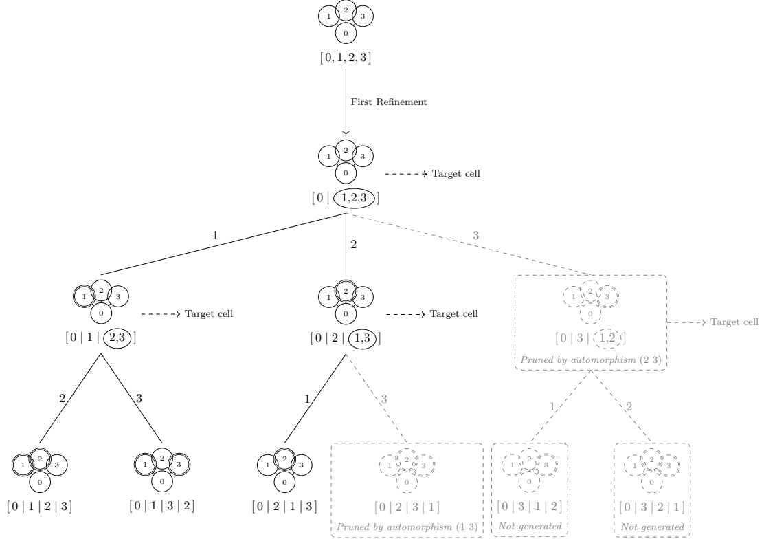
Figure 4.5: Search tree for K_{1,3} with the P_C pruning strategy applied.
