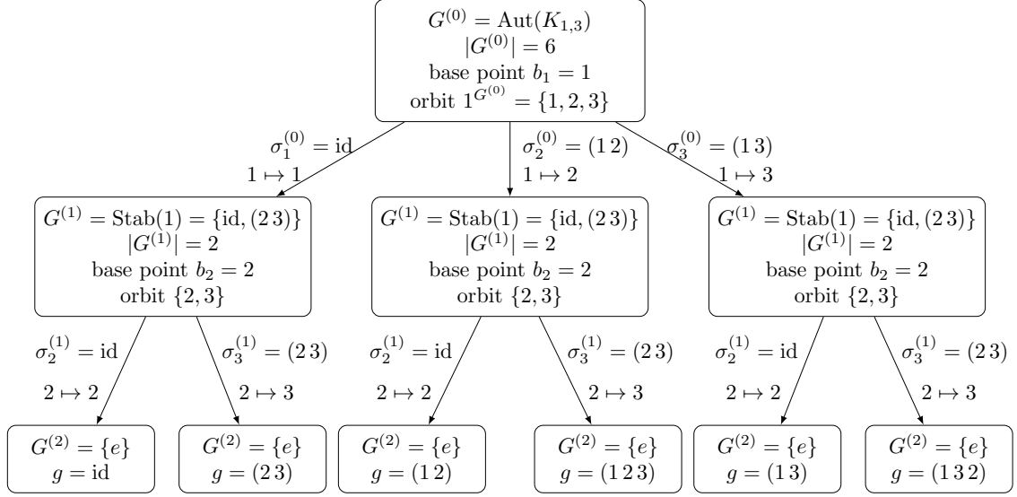
Figure 2.4: Tree associated with the BSGS of \text{Aut}(K_{1,3}) with base (b_1 = 1, b_2 = 2) .
