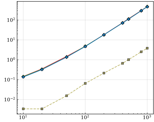
Trees
