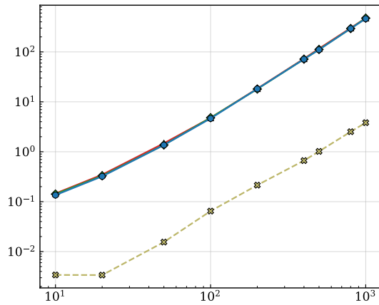
Dense Graphs
