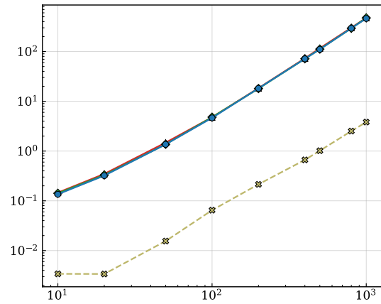
Sparse Graphs
