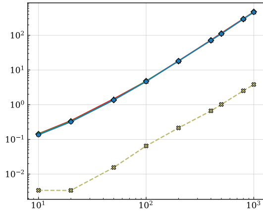
Regular graphs
