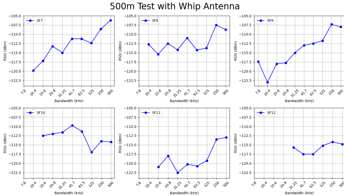
Figure 1.4: 500m Test with Whip Antenna
