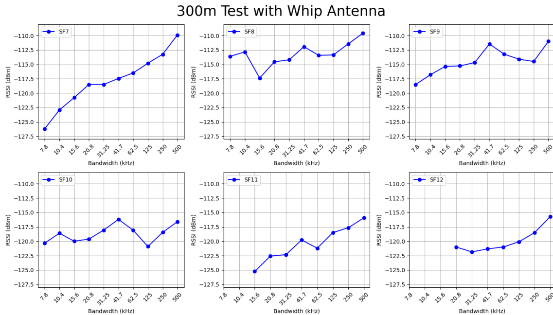
Figure 1.3: 300m Test with Whip Antenna
