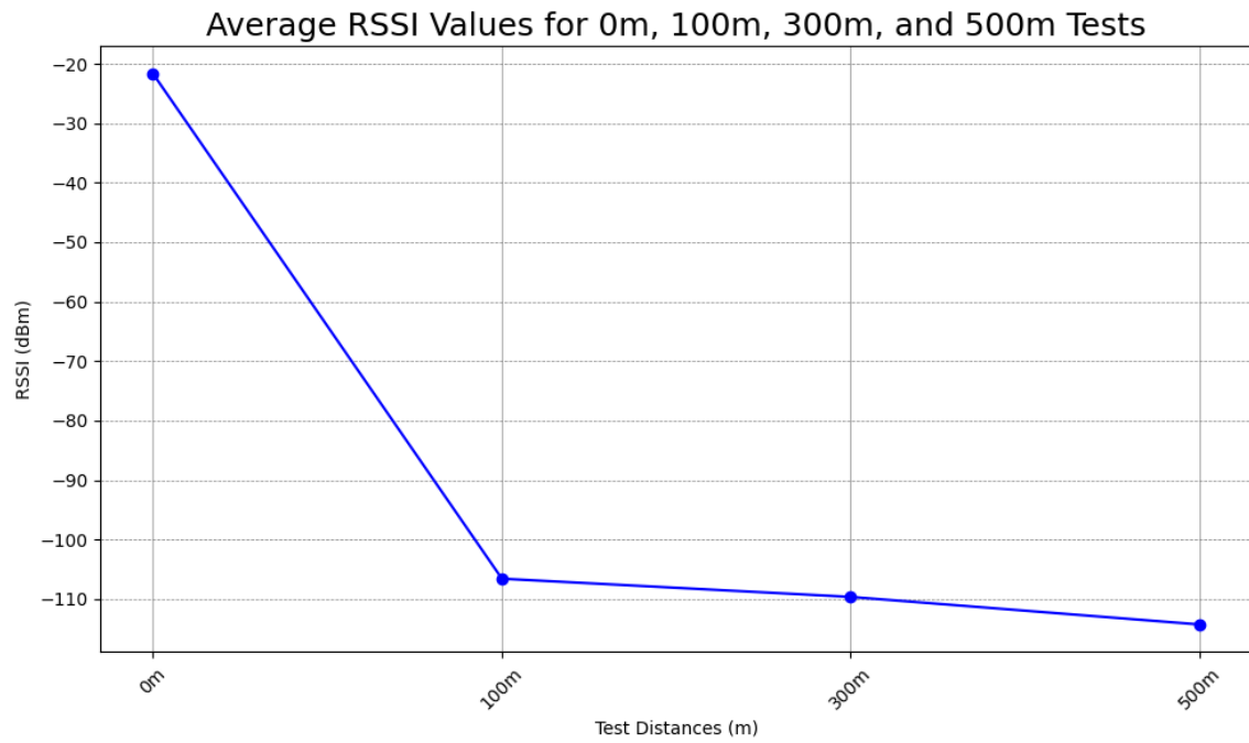
Figure 1.6: Average RSSI Value of Transmissions for Various Test Distances
