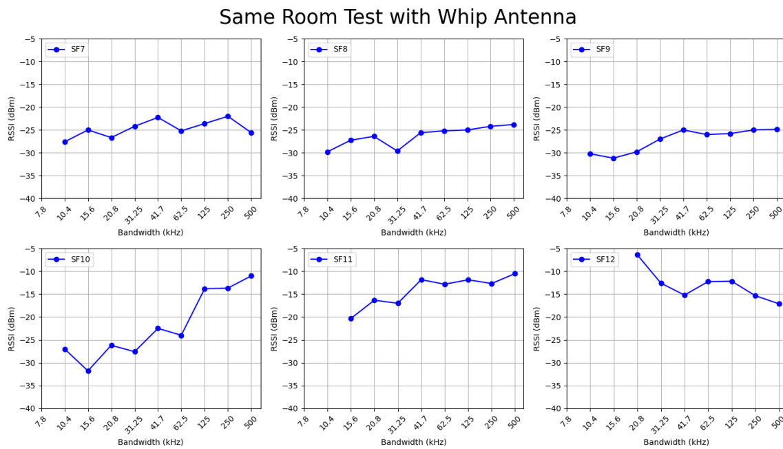
Figure 1.1: Same Room Test with Whip Antenna
