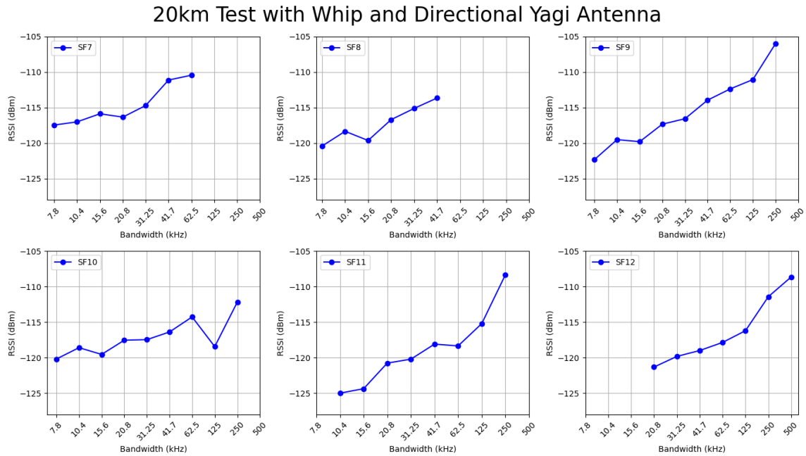
Figure 1.5: 20km Test with Whip and Yagi Antenna
