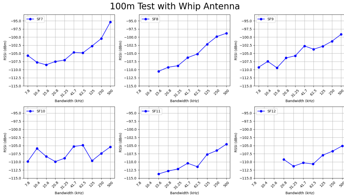
Figure 1.2: 100m Test with Whip Antenna
