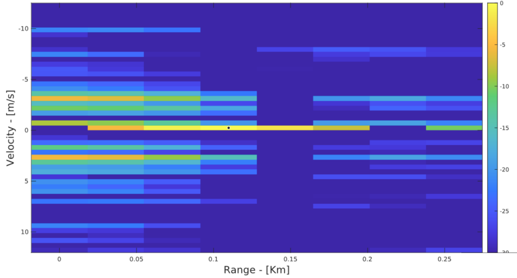
Figure 2.3: Range-doppler map of object at 100m
