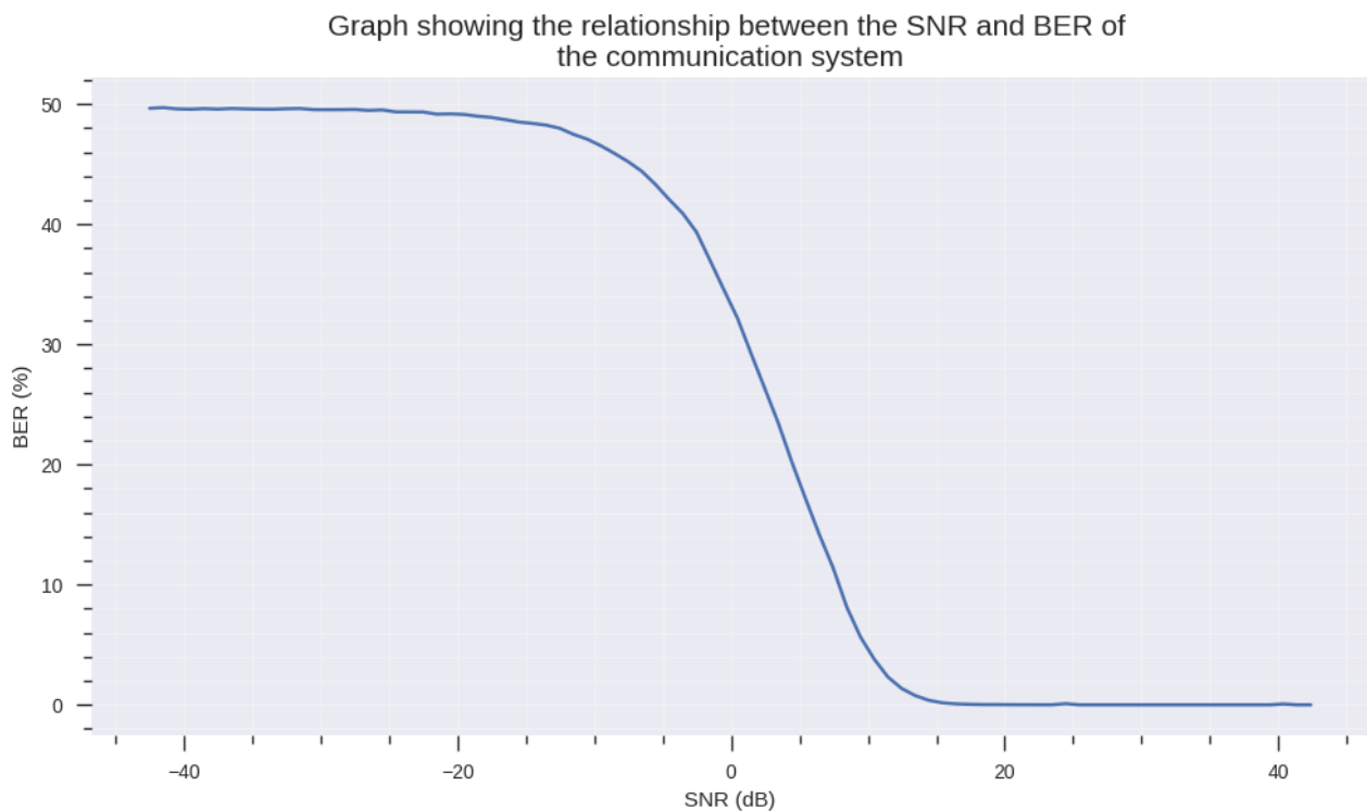
Figure 7.1: Result of cable loopback characterization of communication system
