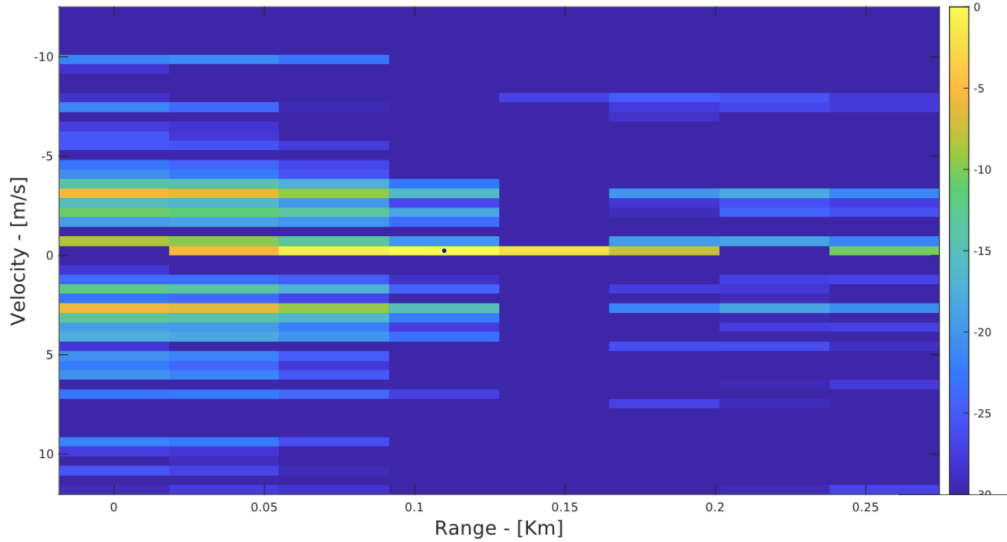
Figure 3.3: Range-doppler map of object at 100m
