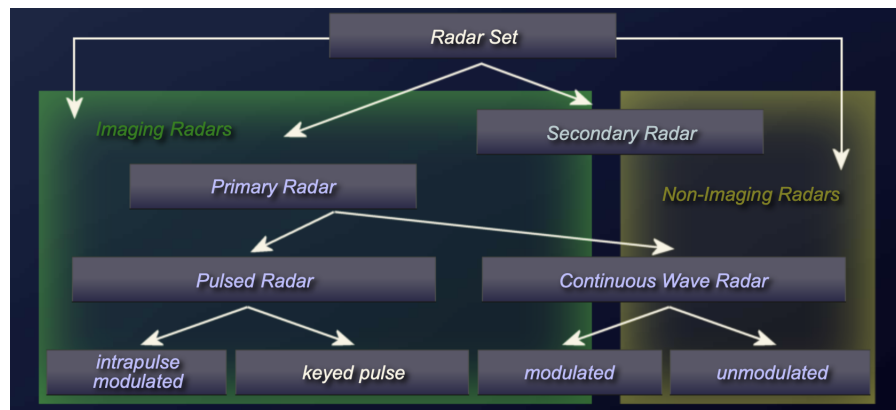
Figure 3.1: Classification of Radar Systems [1]
