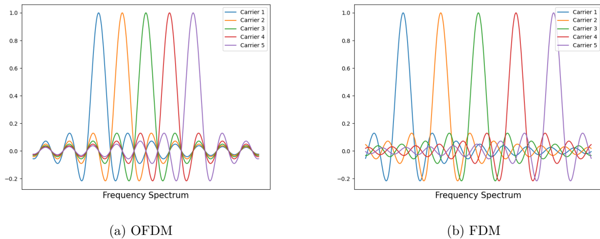
Figure 3.2: OFDM and FDM Waveforms
