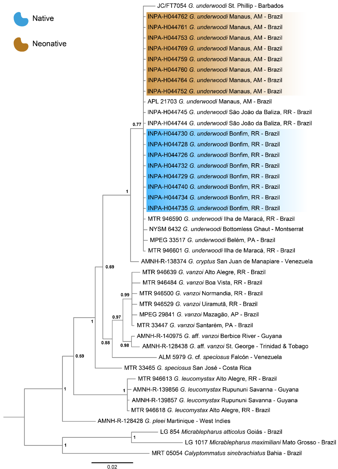
Figure S2. Bayesian Inference of mDNA 16S of Gymnophthalmus underwoodi . Individuals collected in the native population (blue band) and in the neonative population (brown band)
