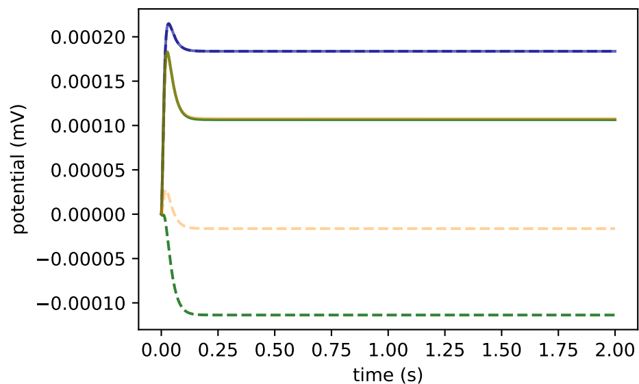
PyRates(--) vs pure Python(-) with 10, 11 and 16 populations
