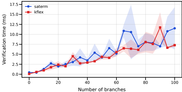
Verification time vs branch count
