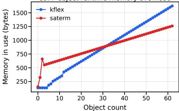
eBPF object runtime memory overhead
