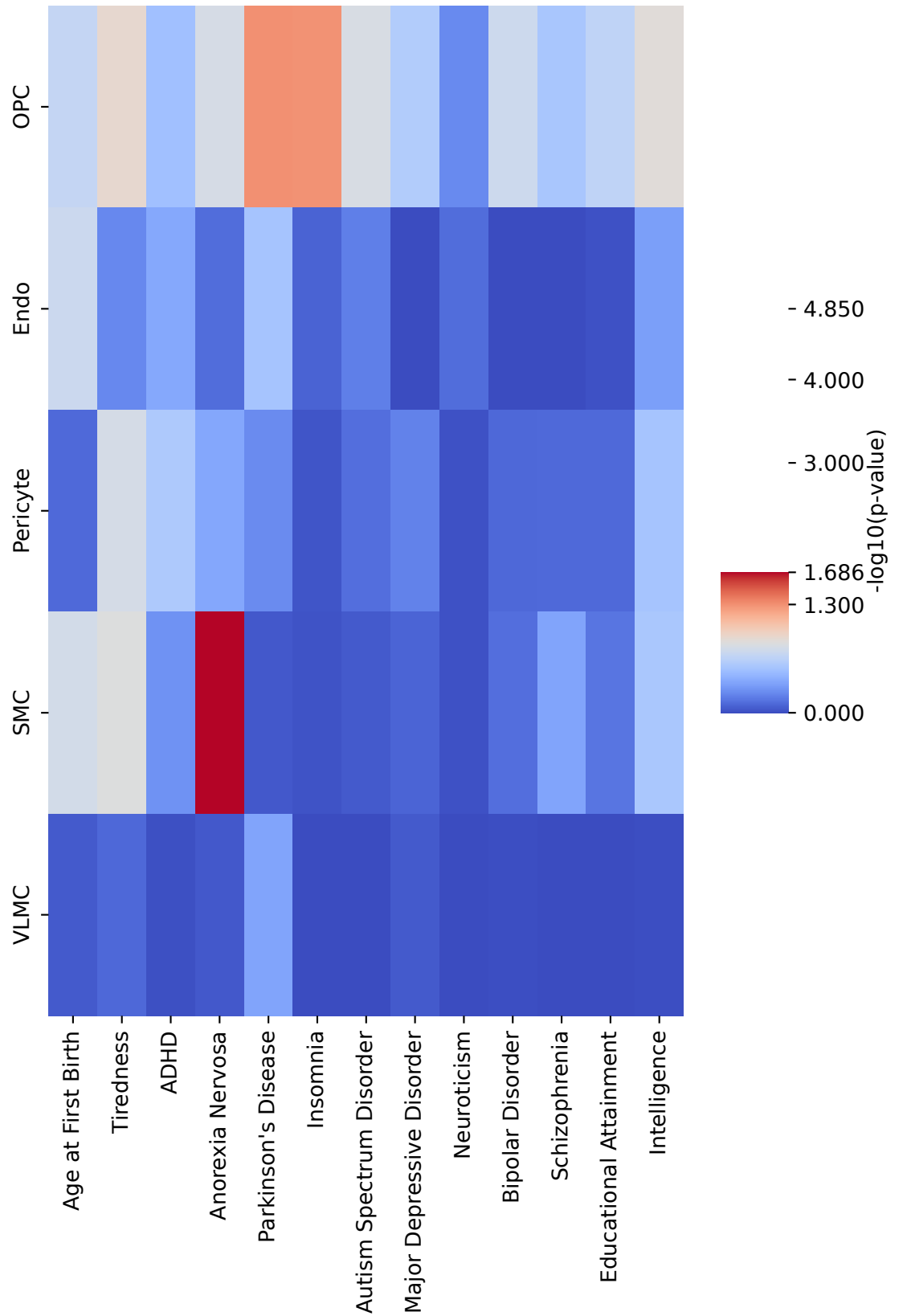
LDSC on Subclass loop anchors
