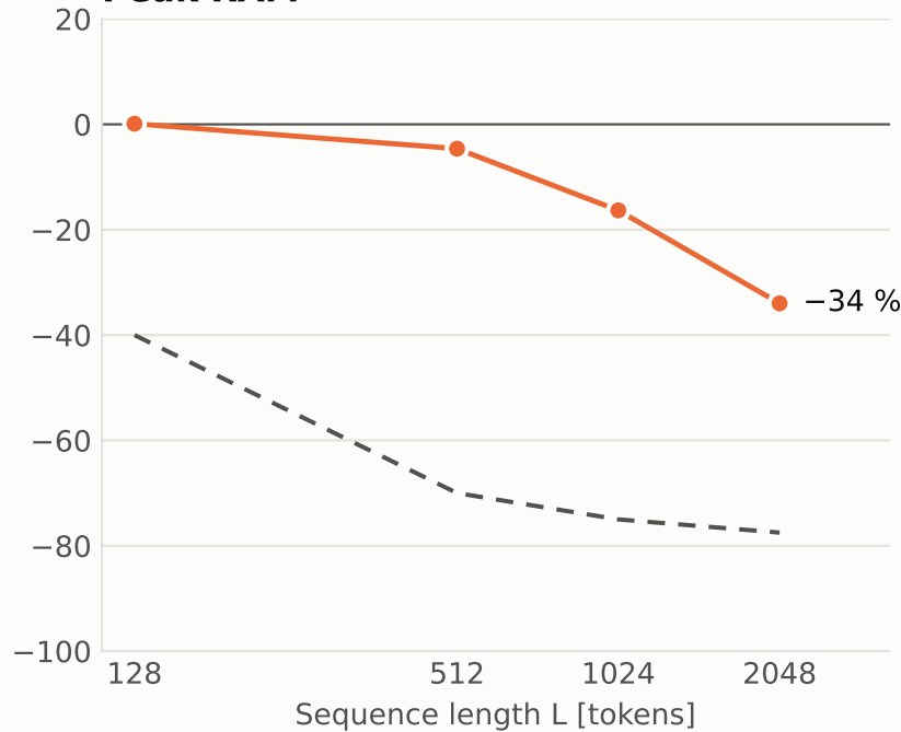
Peak RAM
