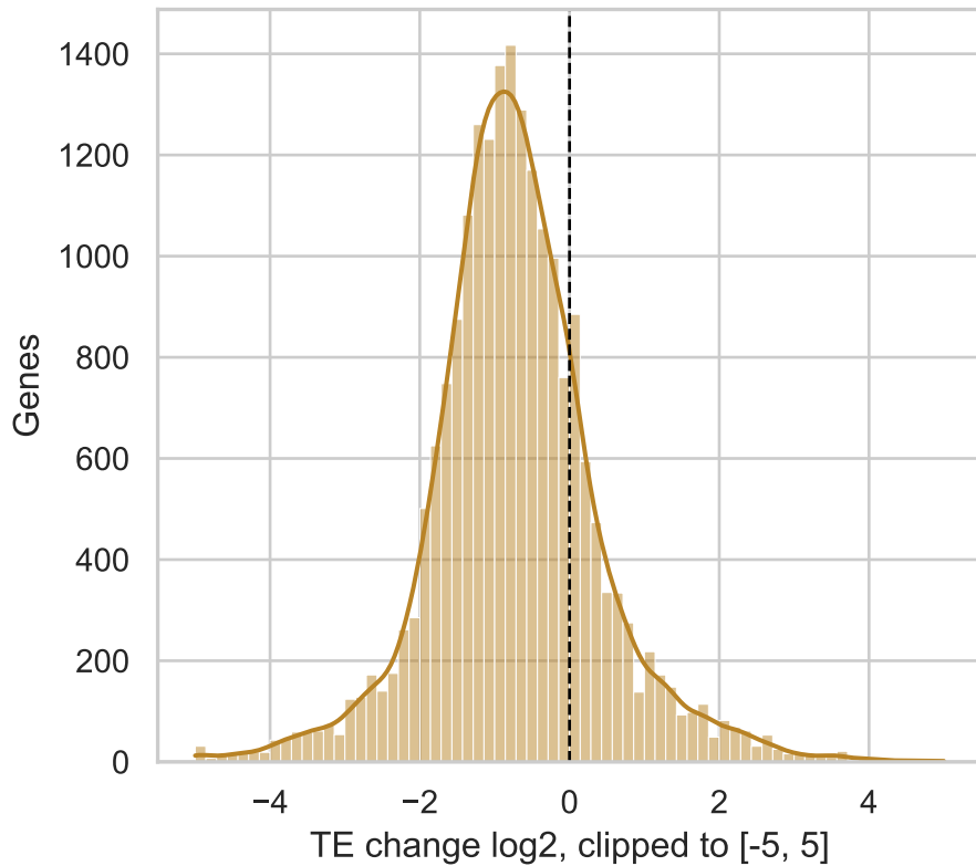
Translation Efficiency Change Distribution
