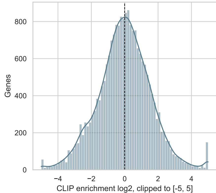
CLIP Enrichment Distribution
