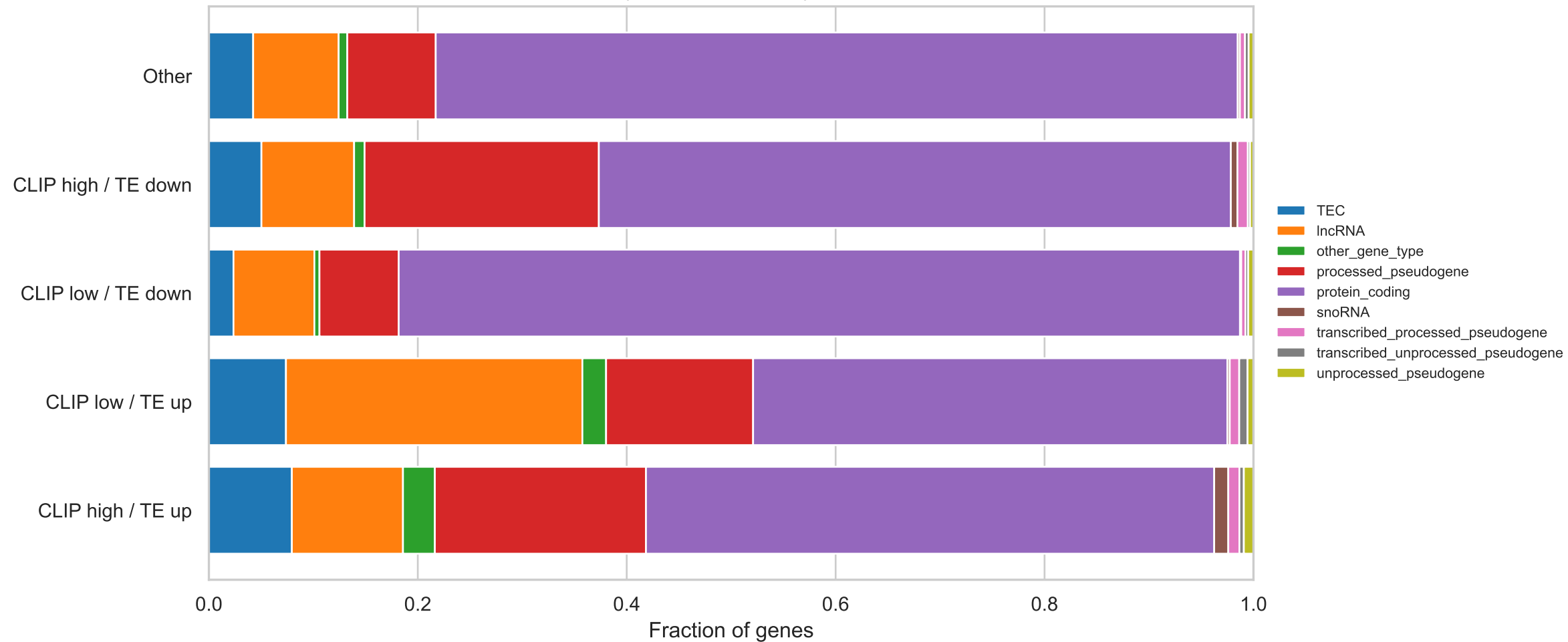
Gene-Type Composition by Quadrant
