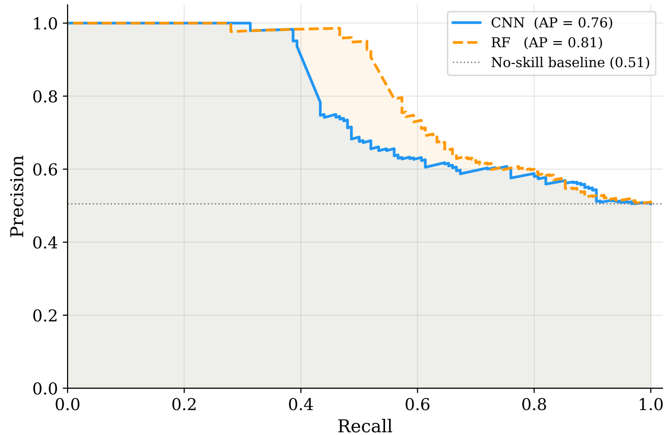
Precision-Recall — Transit Detection
