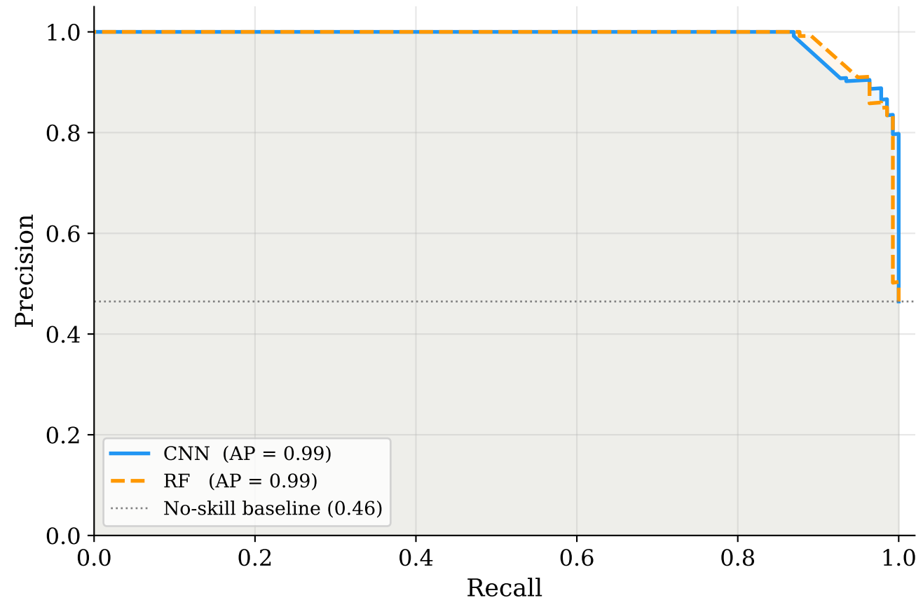
Precision-Recall — Flare Detection
