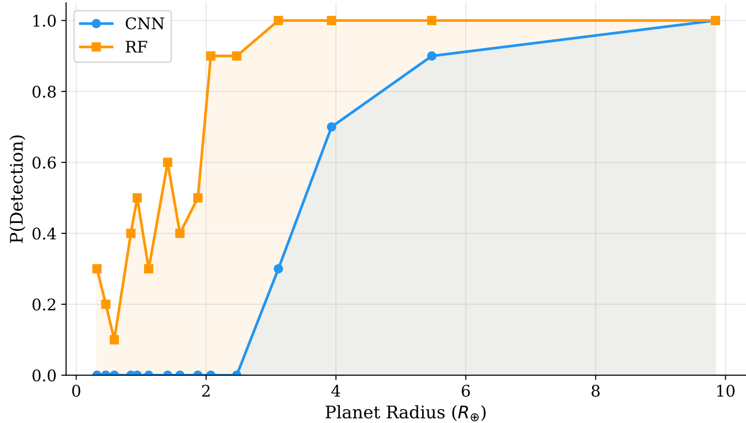
Transit Detection Efficiency vs. Planet Radius
