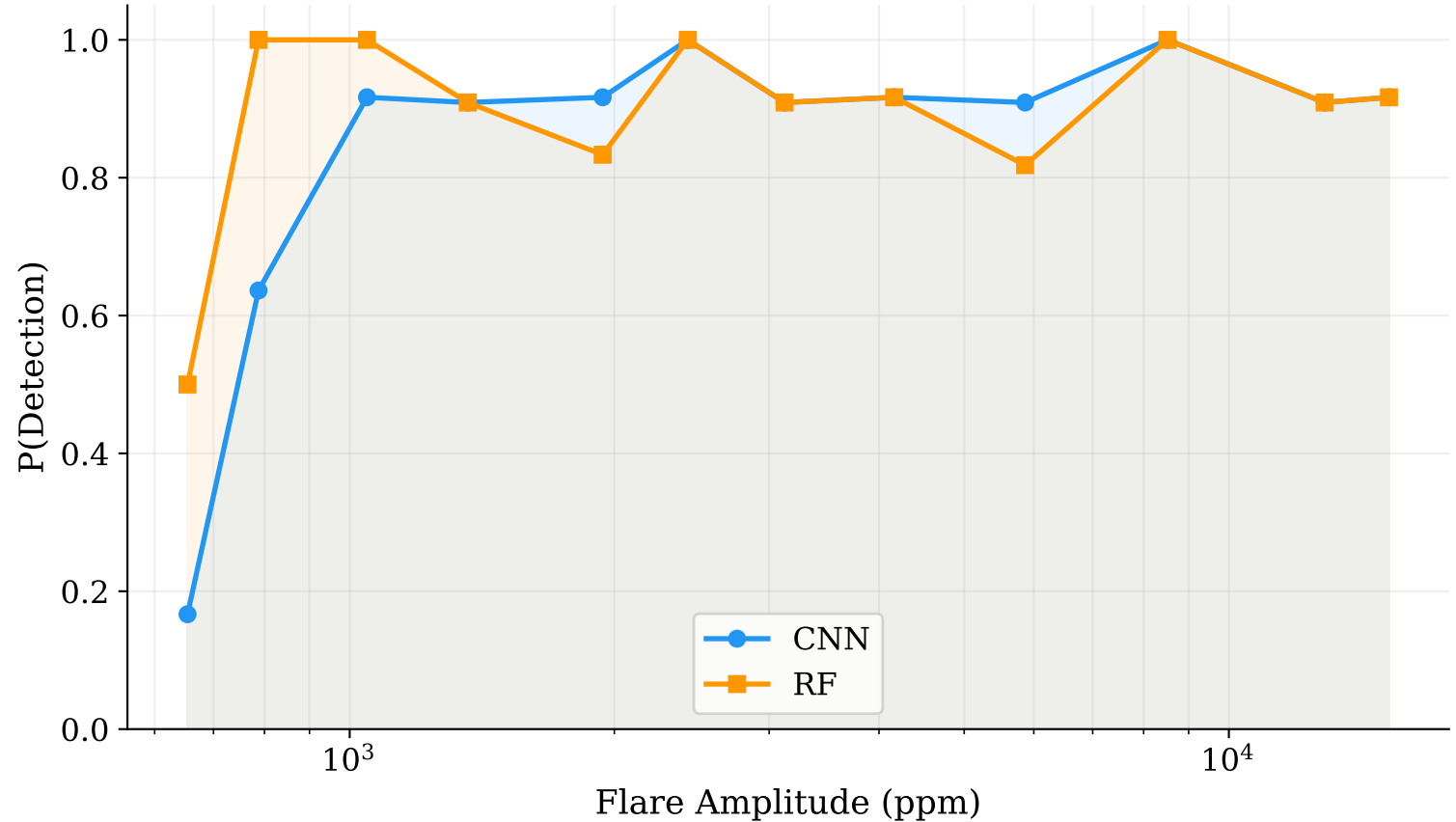
Flare Detection Efficiency vs. Amplitude
