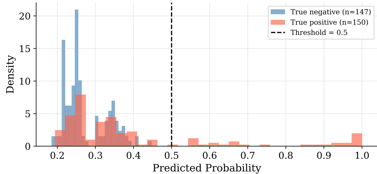
CNN — Transit
