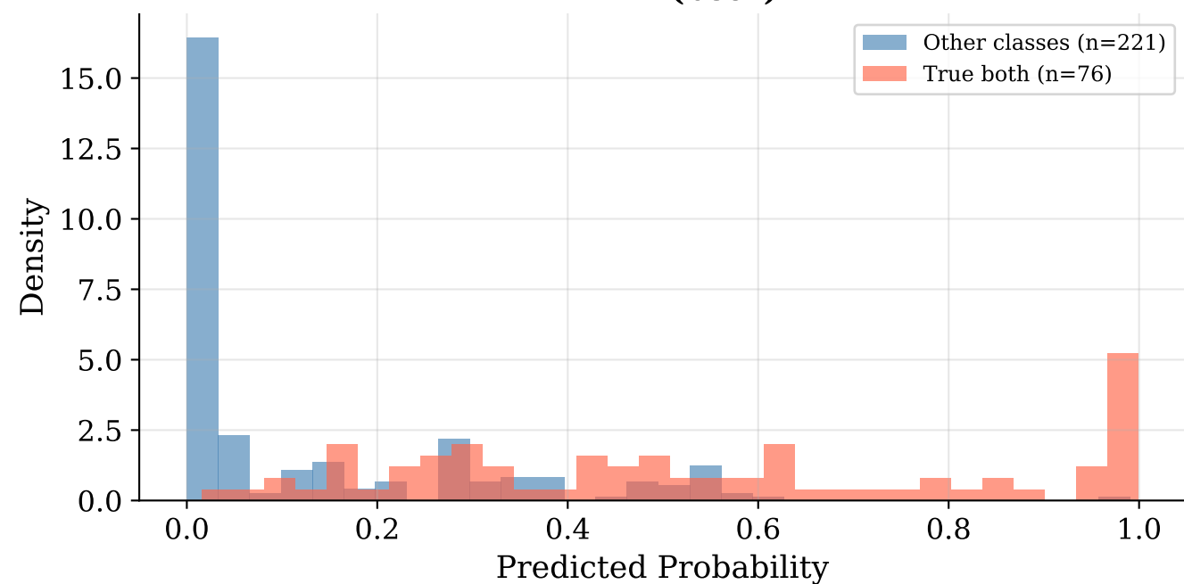
RF — P(both)
