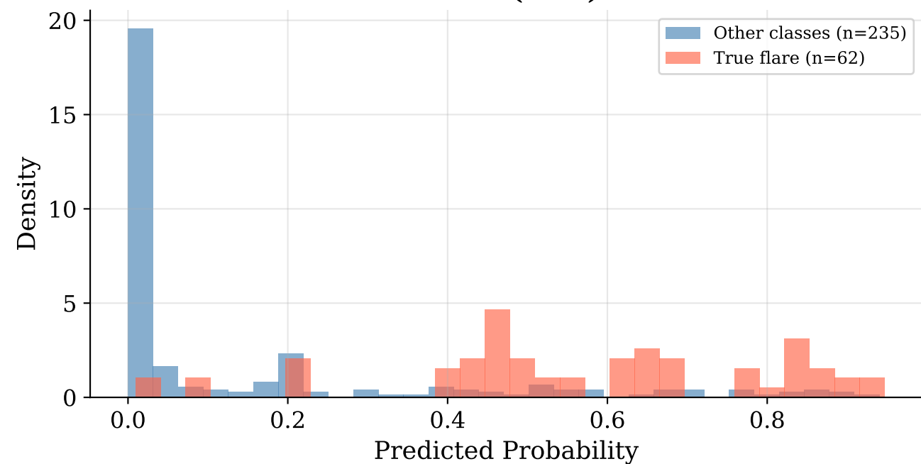
RF — P(both)
