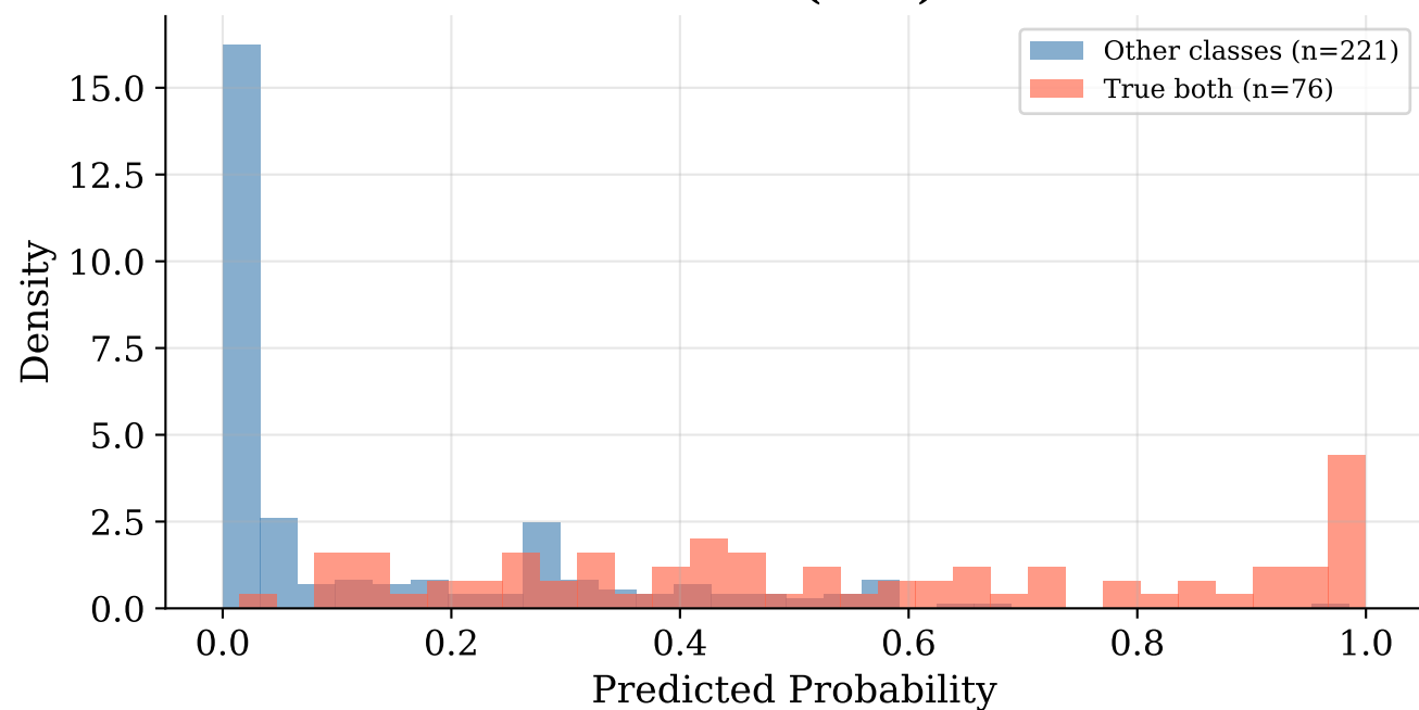
RF — P(both)
