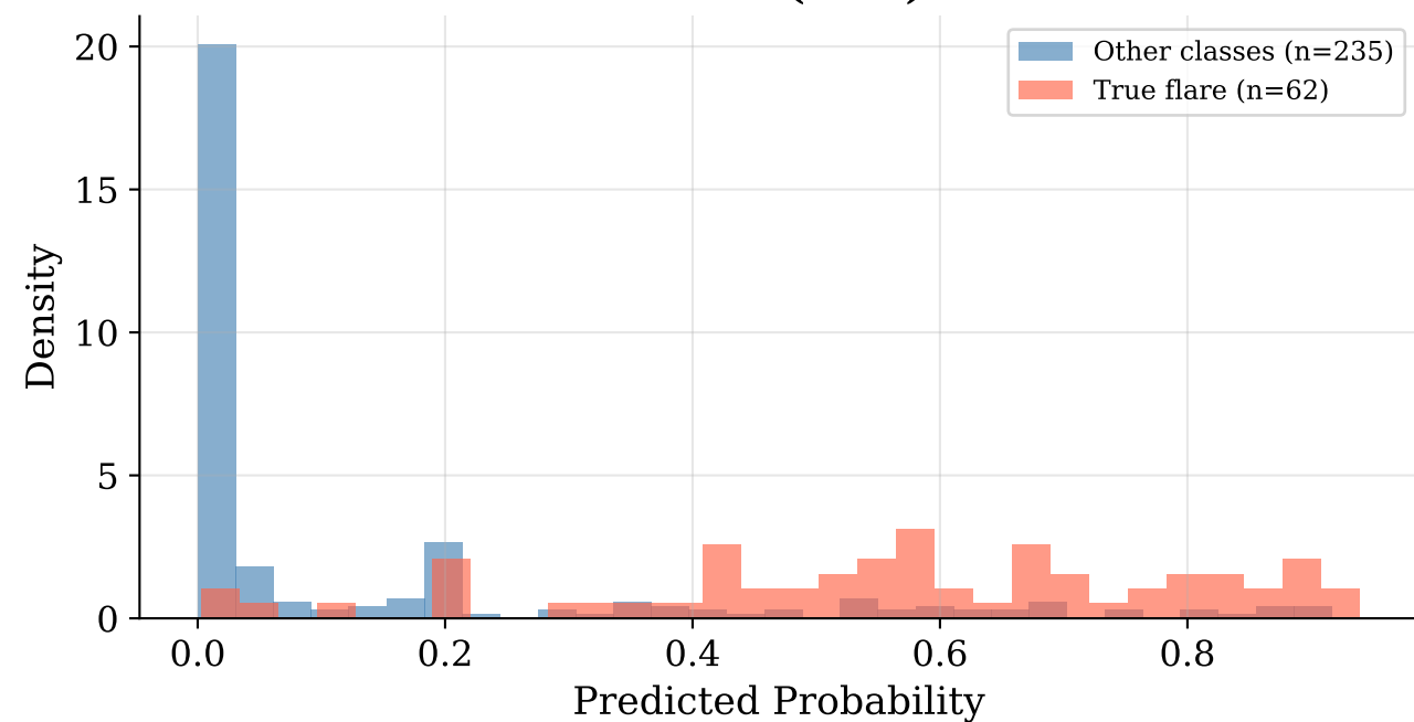
RF — P(both)
