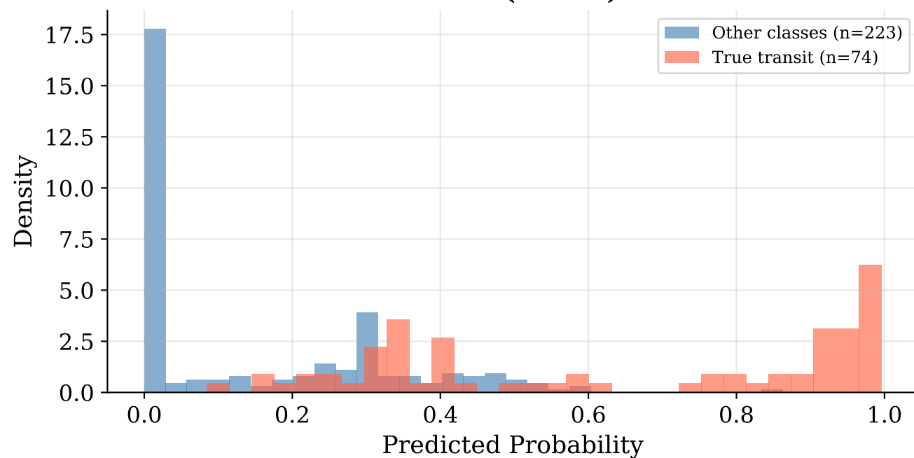
RF — P(transit)
