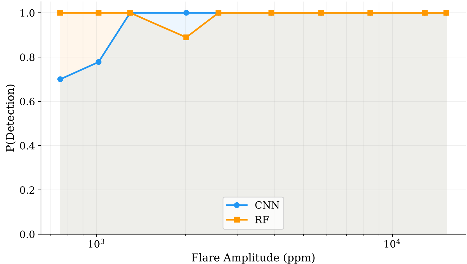
Flare Sensitivity — No Drift Systems
