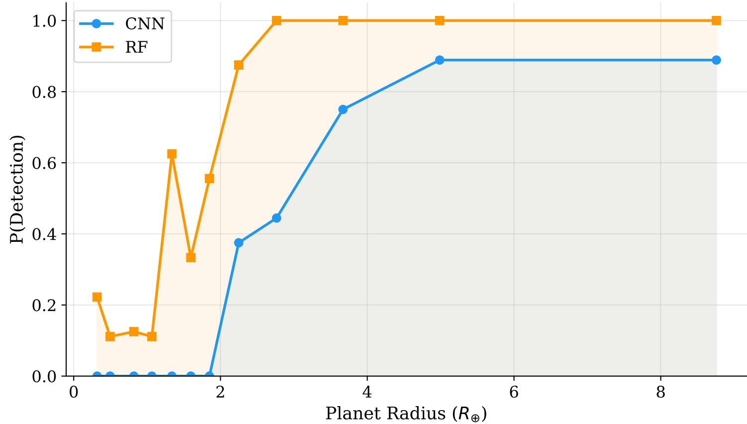
Transit Sensitivity — No Drift Systems
