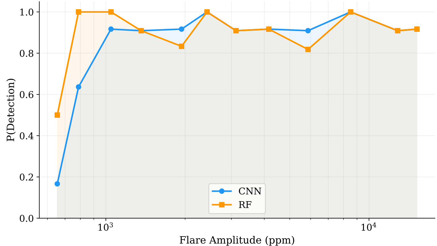
Flare Detection Efficiency vs. Amplitude
