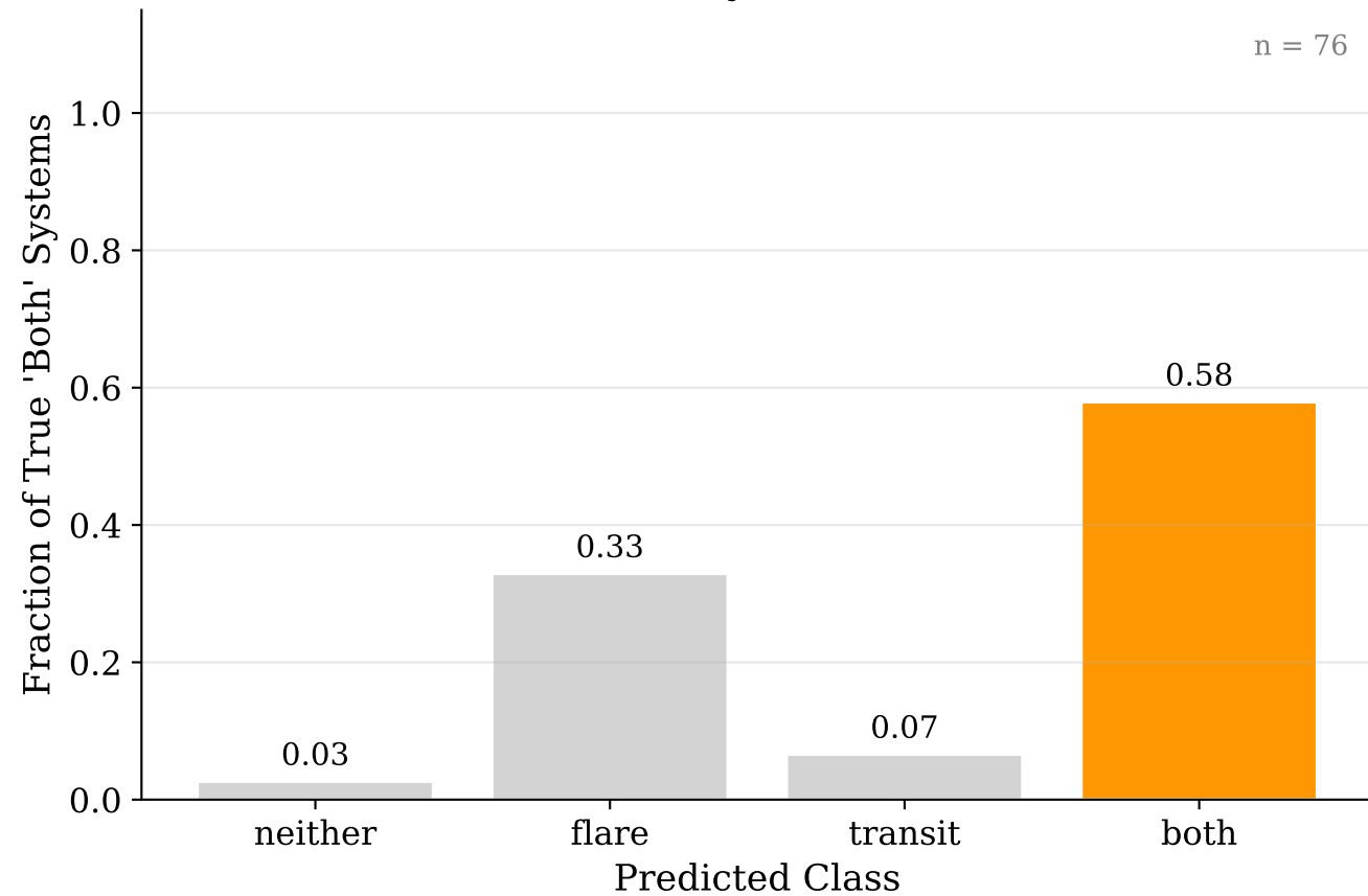
RF — True 'Both' Systems: Predicted As?
