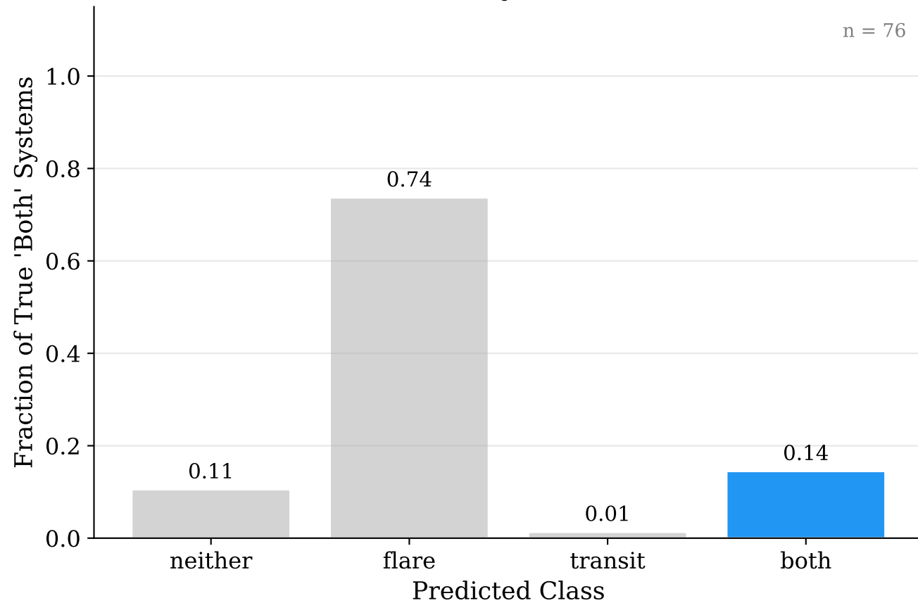
CNN — True 'Both' Systems: Predicted As?
